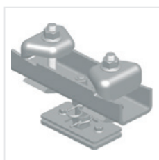
31280 08011 Pendelabhngung Standard / Fixation IPN articul e / I-Beam Bracket, Swivel Adjustment
