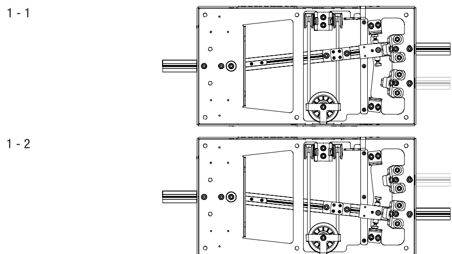
Fig. 9: Track switch 1 to 2 manual – Track switch positions
