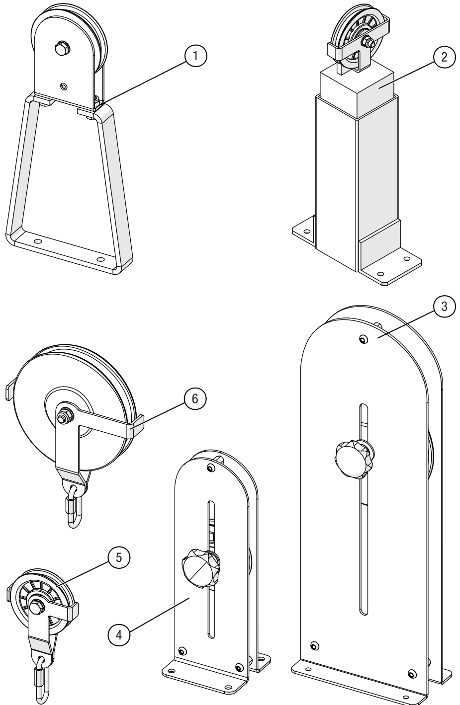
Fig. 28: Manual drive – Floor pulley
