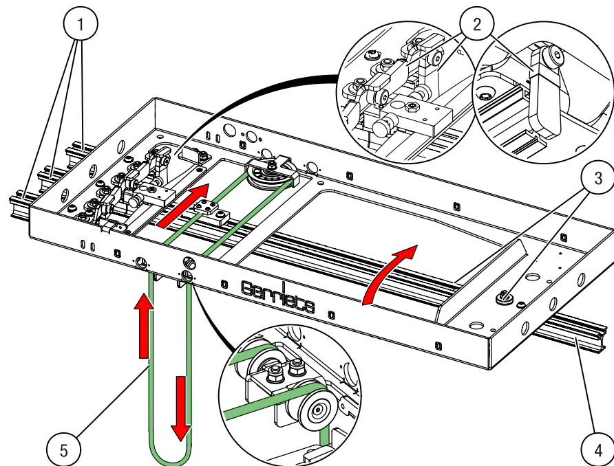
Fig. 5: Manual track switch 1 to 3 (example)
