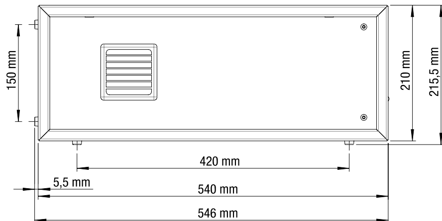
Fig. 39: Side view – G-FRAME 54 control system
