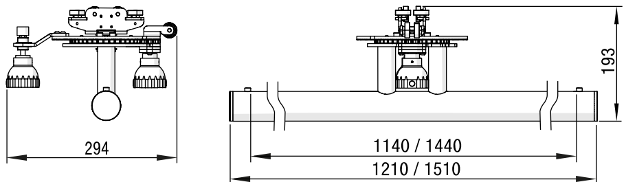
Fig. 35: Dimensions – Swivel pipe 1200 / 1500
