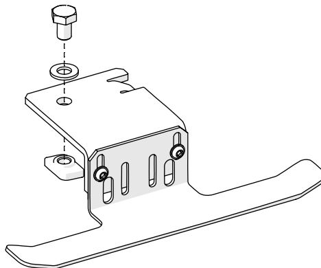
Fig. 25: Accessories – FRICTION DRIVE limit switch arm
