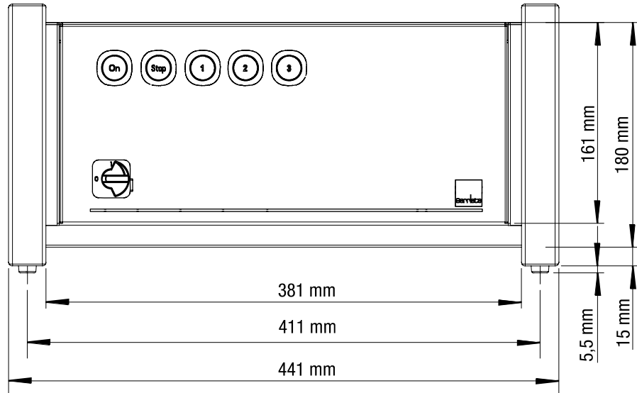
Fig. 38: Front view – G-FRAME 54
