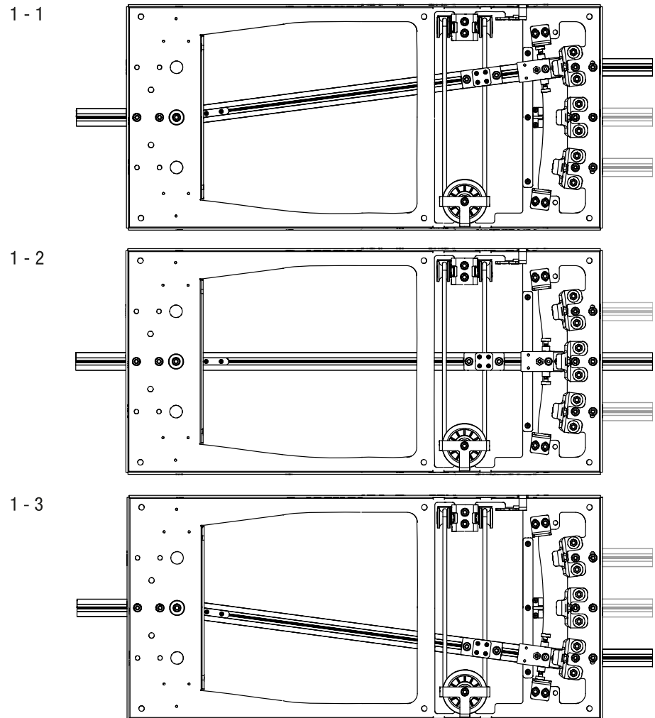
Fig. 8: Track switch 1 to 3 manual – Track switch positions
