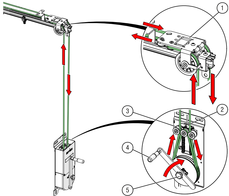
Fig. 27: Manual drive HAND-DRIVE with TRUMPF 95 track system
