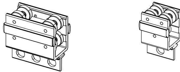
Fig. 14: Runner 4 + 4 (left) and runner 4 + 2 (right)
