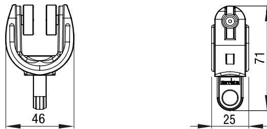
Fig. 29: Dimensions – 2-wheel-runner
