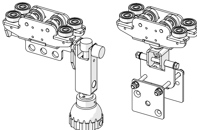
Fig. 15: HD braked runner (left) and scenery runner (right)
