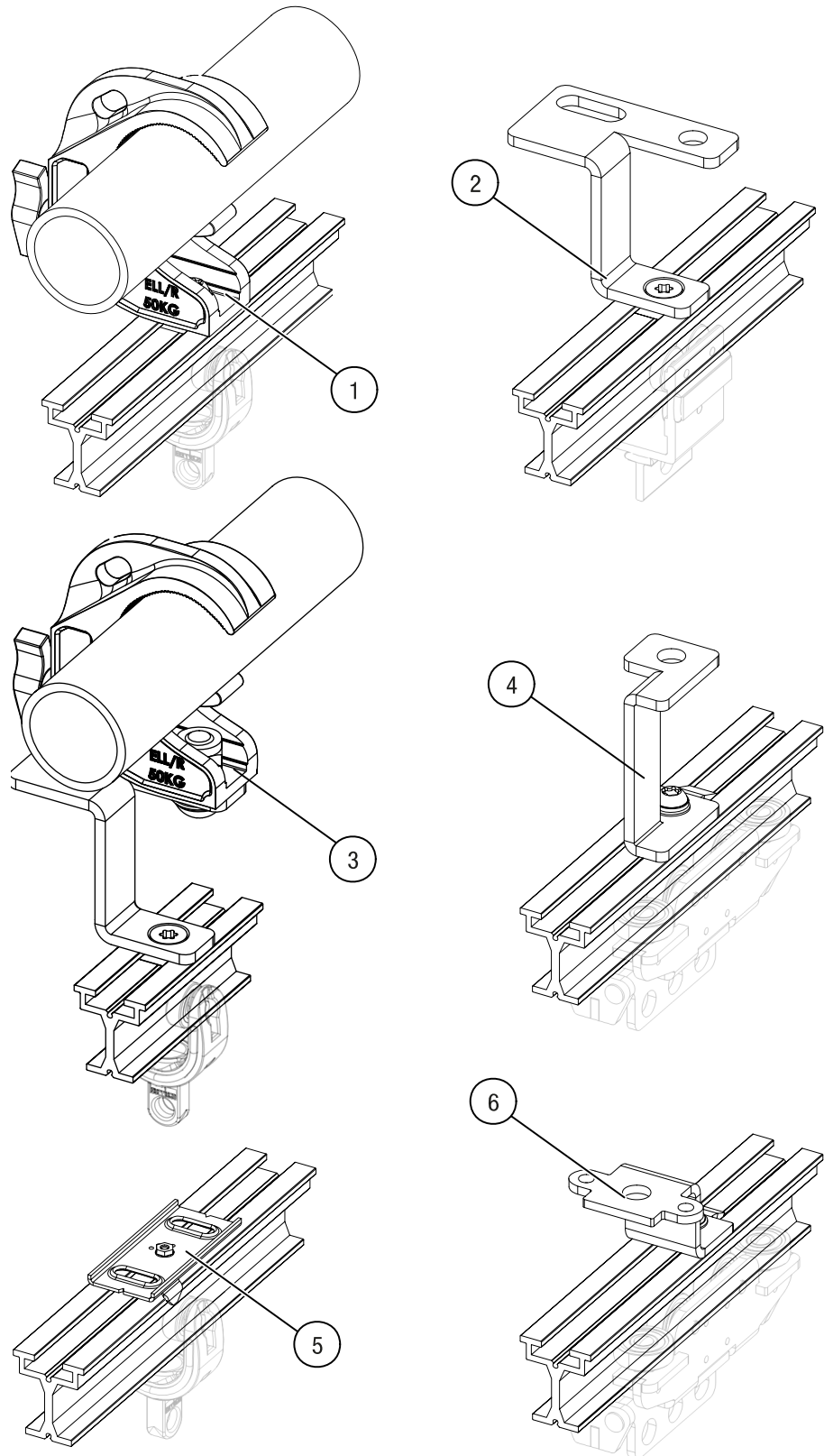
Fig. 11: TRUMPF 95 – Suspension variants
