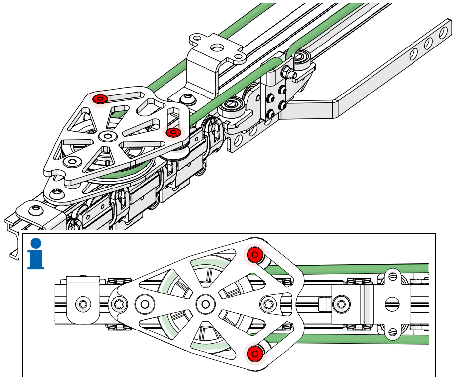
Fig. 73: Side cord operation – Final cord positioning at the return pulley
