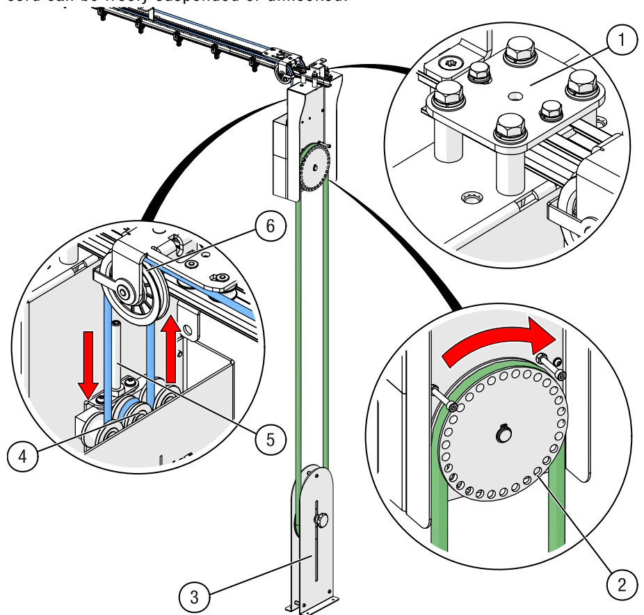
Fig. 26: Manual drive ROPE DRIVE with hemp rope floor pulley and TRUMPF 95 track system
