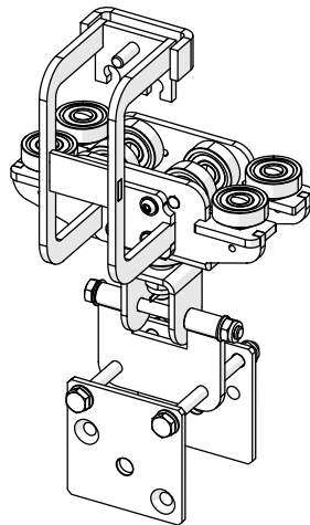
Fig. 22: Master runner HD as scenery runner with scenery attachment for double top cord operation
