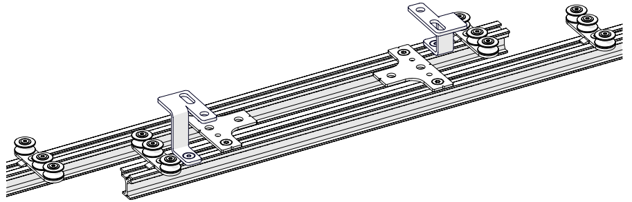
Fig. 90: Top cord operation – Track change on double track system
