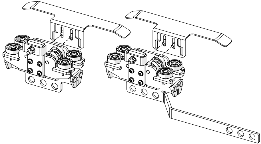
Fig. 17: TRUMPF 95 master runner HD with limit switch arm (left) and TRUMPF 95 master runner HD with overlap arm and limit switch arm (right)
