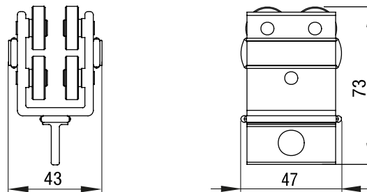
Fig. 30: Dimensions – 4-wheel-runner
