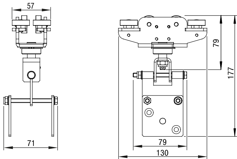
Fig. 34: Dimensions – Scenery runner
