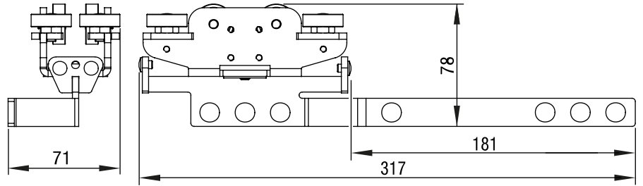
Fig. 33: Dimensions – HD master runner with overlap arm
