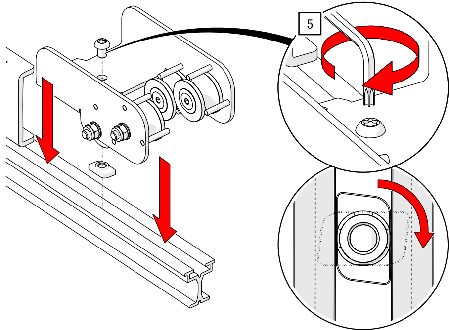
Fig. 108: Double top cord operation – Mounting the double top cord operation head pulley
