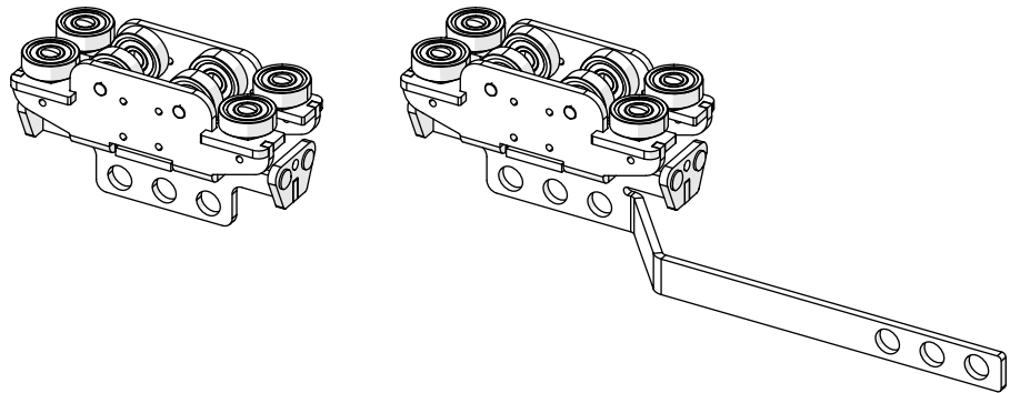
Fig. 13: Master runner HD (left) and master runner HD with overlap arm (right)
