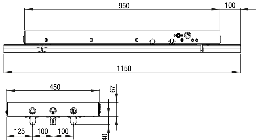
Fig. 37: Dimensions – Track switch 2 on 3 and 1 on 3
