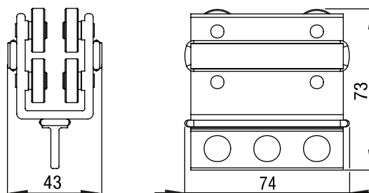
Fig. 31: Dimensions – 4x4-runner
