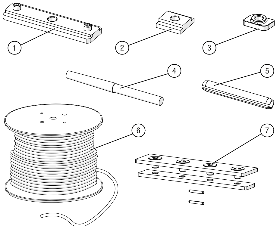
Fig. 23: Accessories – TRUMPF 95 track system
