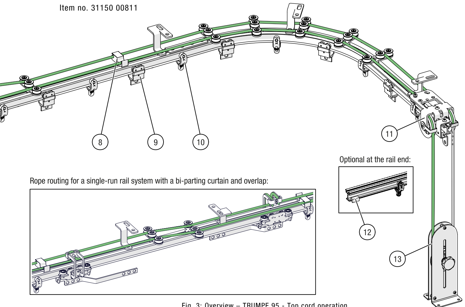
Fig. 3: Overview – TRUMPF 95 - Top cord operation
