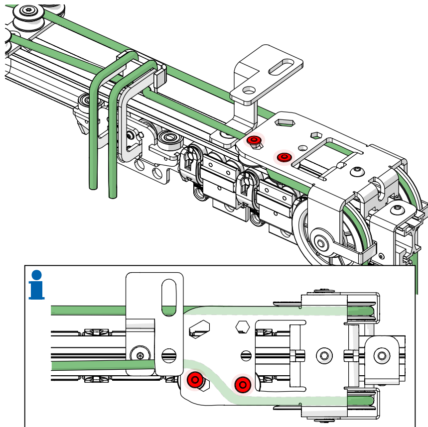
Fig. 85: Top cord operation – Final cord positioning at the head pulley
