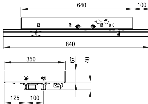
Fig. 36: Dimensions – Track switch 1 to 2
