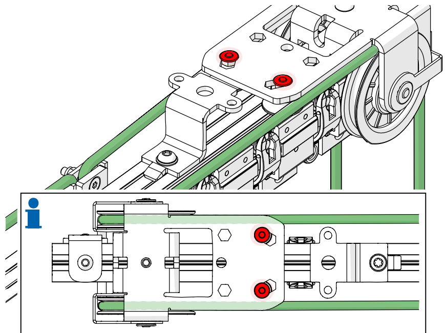
Fig. 72: Side cord operation – Final cord positioning at the head pulley
