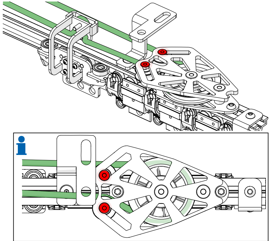
Fig. 86: Top cord operation – Final cord positioning at the return pulley
