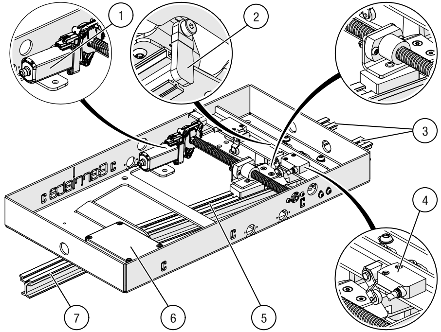
Fig. 6: Track switch 1 to 2 electrical (example)
