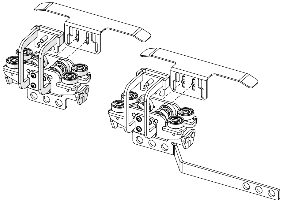
Fig. 19: TRUMPF 95 master runner HD with limit switch arm (left) and master runner HD with overlap arm and limit switch arm (right)
