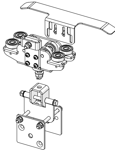
Fig. 18: Master runner HD as scenery runner with scenery attachment with limit switch arm
