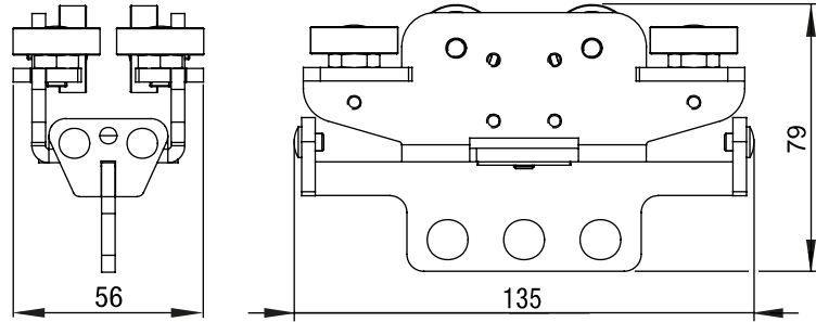
Fig. 32: Dimensions – HD master runner
