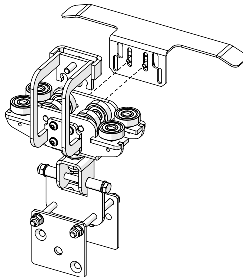
Fig. 20: Master runner HD as scenery runner with scenery attachment with limit switch arm
