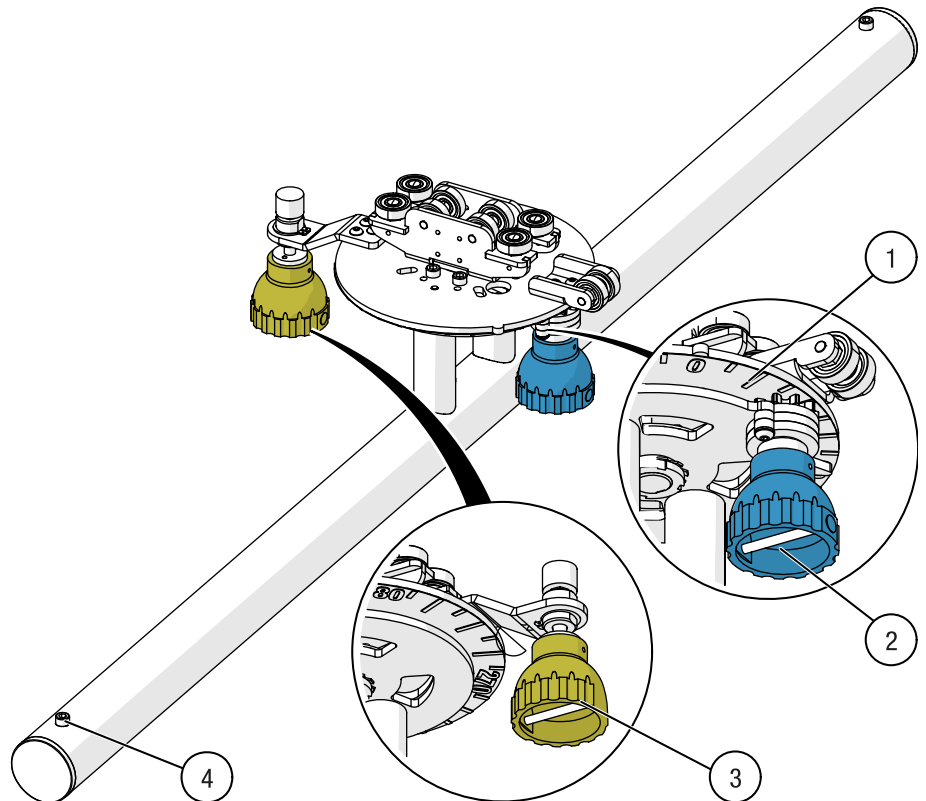
Fig. 16: TRUMPF 95 – Swivel pipe
